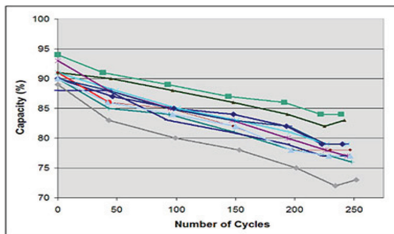
Chart 1: Capacity drop as part of cycling
