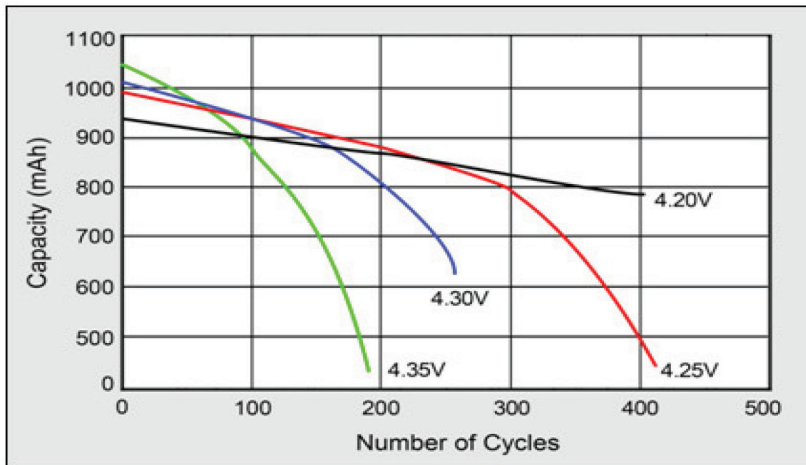
Figure 2: Cycle count versus charge voltage
