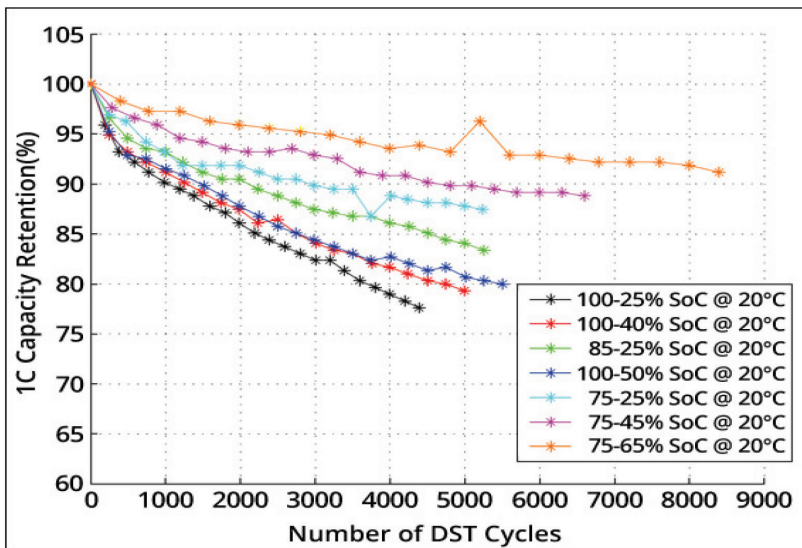
Figure 3: Capacity loss versus % charge / % discharge dynamic cycling
