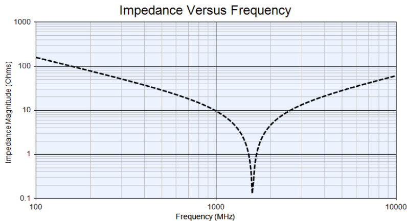
Figure 3 - Impedance & ESR vs. Frequency for 10pF MLCC
