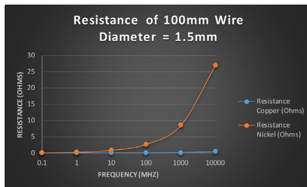
Figure 4 - Resistance of Copper & Nickel Wire
