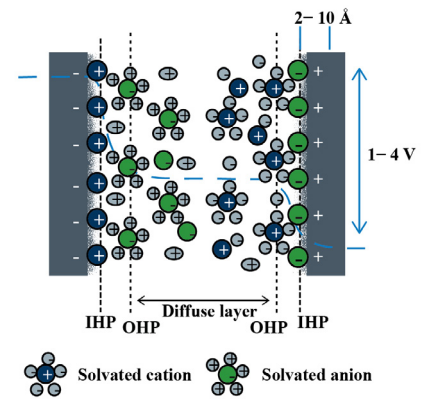
Figure 1: Diagram of EDLC illuminating the double-layer with the inner Helmholtz plane (IHP) and the outer Helmholtz plane (OHP).
